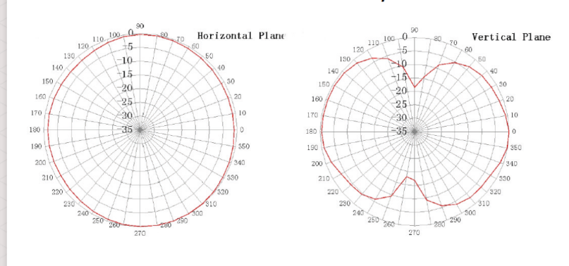
2D - RADIATION PATTERN H/V
